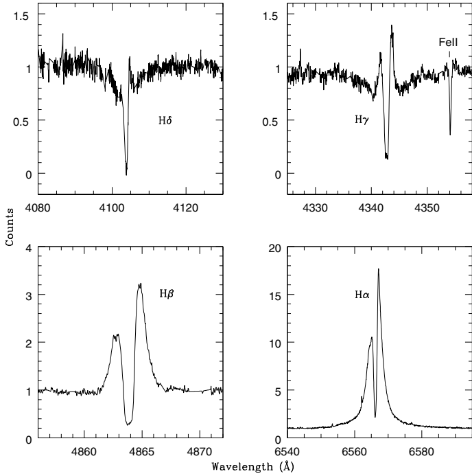
Fig. 2. Balmer lines in the spectrum of S 23.
