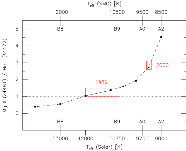
Fig. 3. Effective temperature dependence of the line ratio \text{MgII } \lambda 4481 over \text{HeI } \lambda 4472 calculated from model stellar atmospheres with \log g = 2.5 at solar abundances. The behaviour between spectral type and effective temperature taken from Evans & Howarth (2003) is indicated in the bottom label for solar abundance, and in the top label for SMC abundance. The two boxes indicate the observed ratios with their errors for the ZSW spectrum taken in 1989 and our spectrum taken in 2000, respectively.
