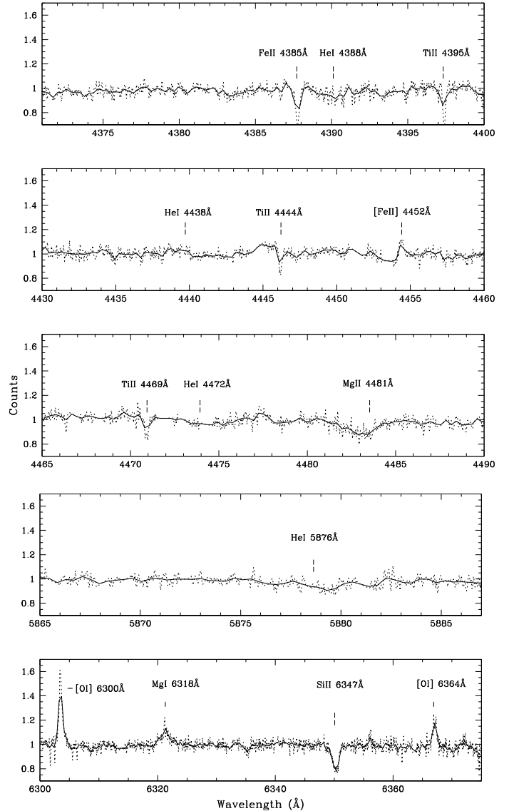
Fig. 1. Parts of the rectified FEROS spectrum (dashed lines) showing the regions around several expected HeI lines. For better visualization, we convolved the FEROS data to a resolution of R = 4900 as was used by ZSW (solid lines).
