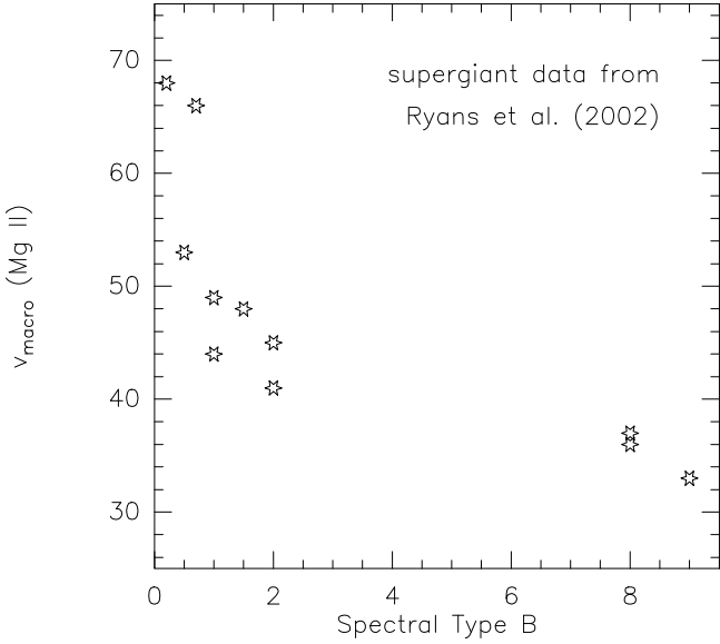
Fig. 5. Maximum velocity caused by macro-turbulence to the MgII \lambda 4481 line for a sample of B-type supergiants. The data are taken from Ryans et al. (2002).
