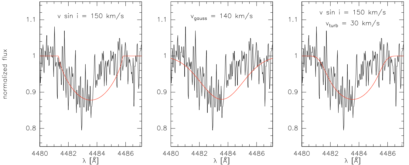
Fig. 4. Fitting process of the MgII \lambda 4481 line with a pure rotation profile ( left panel ), a pure Gaussian profile ( mid panel ), and our best fit model ( right panel ) with a profile consisting mainly of stellar rotation plus some macro-turbulence.
