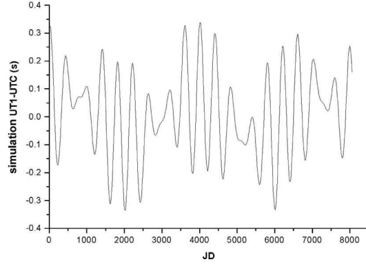
Fig. 1. Simulated data UT1 - UTC containing harmonic terms with periods of 1.0, 1.2, 2.0 and 9.0 years.
