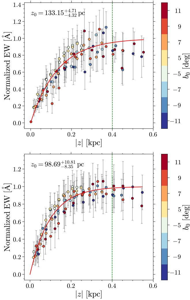
Fig. 15. Determination of the scale height of the \lambda 862 carrier by the DIB measurements with 4^\circ \leq |b| \leq 12^\circ , and upper panel : 240^\circ \leq \ell \leq 330^\circ ; lower panel : toward all available longitude directions, respectively. The data points at different latitude slabs are coloured according to the central latitude values ( b_0 ). The dashed green line indicates z = 0.4 kpc. The red curve in the upper panel is the fit to data points with z \leq 0.4 kpc, while in the lower panel, the red curve is the fit to all the data points.
