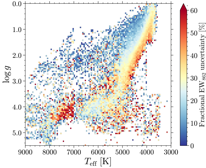
Fig. 3. Kiel diagram as a function of the fractional EW_{862} uncertainty ( \text{err}(EW_{862})/EW_{862} ) for a subsample with QF < 5 . The mean EW_{862} uncertainty is calculated in 50 \text{ K} \times 0.05 \text{ dex} bins.
