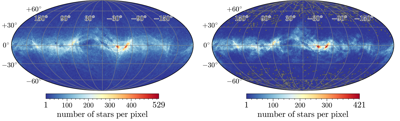
Fig. 1. (Left panel:) Galactic distribution of the 476 117 DIBs \lambda 862 in Gaia DR3. The spatial resolution is 1.8^\circ per HEALpixel (level 5). The colour scale indicates the number of measurements per pixel. (Right panel:) The subset of 236 836 sources with high-quality measurements ( QF \leq 2 , see Sect. 3).
