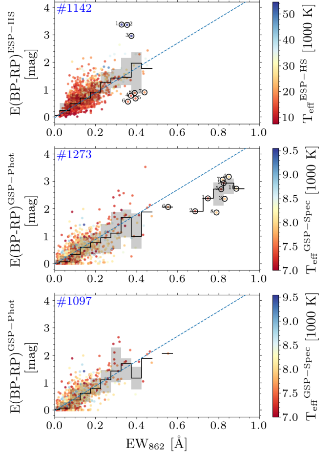
Fig. 9. E(\text{BP} - \text{RP}) vs. EW_{862} of the DIB \lambda 862 derived for the HQ sample by GSP-Spec for hot stars. The colour code follows the effective temperature derived by ESP-HS or GSP-Spec. The running median and interquartile (15 to 85 %) are represented by a black step curve and the shaded area, respectively. The relation derived for the cooler stars is shown by the broken blue line. Upper panel: Reddening derived using the ESP-HS module for stars hotter than 7 500 K. The outliers are identified with black circles and numbers. Middle panel: E(\text{BP} - \text{RP}) from GSP-Phot for targets hotter than 7 000 K according to GSP-Spec only. Lower panel: E(\text{BP} - \text{RP}) from GSP-Phot, and hotter than 7 000 K according to GSP-Spec and GSP-Phot. Numbered black circles denote the outliers which are discussed in the main text, with their parameters listed in Table A.1.
