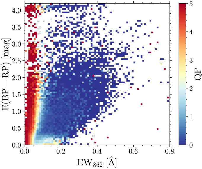
Fig. 2. Equivalent width vs. E(BP - RP) for the DIB \lambda 862 sample coloured by the mean QF calculated in 0.01 \text{ Å} \times 0.05 \text{ mag} bins.
