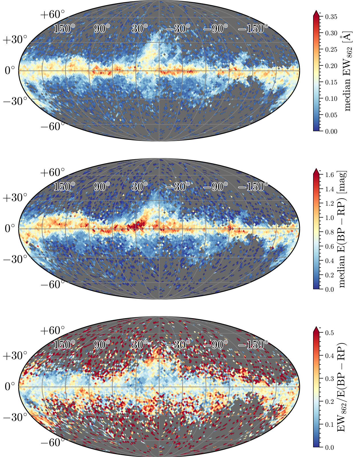
Fig. 6. Comparison between the median EW_{862} of the DIB \lambda 862 (upper panel), the median E(BP - RP) (middle panel), and the ratio EW_{862}/E(BP - RP) (lower panel) at HEALPix level 5 in the Mollweide projection.
