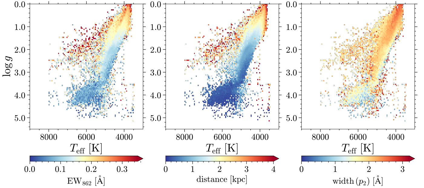
Fig. 5. Mean EW 862 (left panel), heliocentric photogeometric distance from Bailer-Jones et al. (2021) (middle panel), and the width ( p_2 , right panel), calculated in 50 K \times 0.05 dex bins, as a function of the Kiel diagram, respectively.
