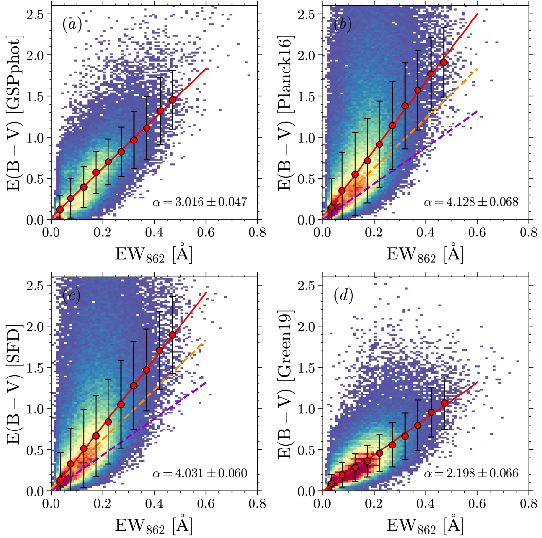
Fig. 8. Correlations between EW_{862} and E(B - V) derived from different extinction maps: (a) GSP-Phot, (b) Planck Collaboration et al. (2016), (c) Schlegel et al. (1998), and (d) Green et al. (2019). The colours in each panel show the target number per 0.01 \text{ \AA} \times 0.02 \text{ mag} bin. The colour bar is the same as in Fig. 7. The red circles are the median values taken in EW_{862} bins from 0 to 0.5 \text{ \AA} with a step of 0.05 \text{ \AA} . The red lines are linear fits to the red dots in each panel, respectively. The fitting gradients ( \alpha ) and their uncertainties are indicated. They are also listed in Table 3. The orange and violet dashed lines in (b) and (c) are the fit results to GSP-Phot and Green et al. (2019), respectively.
