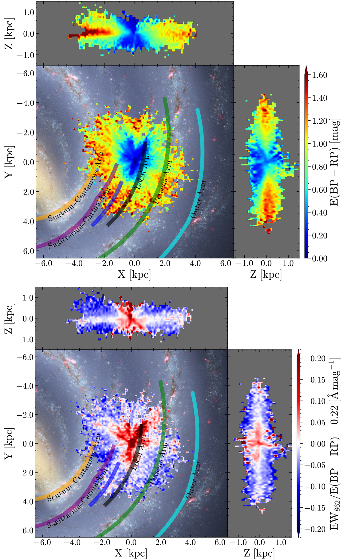
Fig. 12. Same as Fig. 11, but for E(\text{BP} - \text{RP}) from GSP-Phot (upper panel), and the ratio of \text{EW}_{862}/E(\text{BP} - \text{RP}) (lower panel), subtracting 0.22, the inverse of the linear gradient fitted in Fig. 7. Only 55 080 sources in the HQ sample with E(\text{BP} - \text{RP}) measurements are used.
