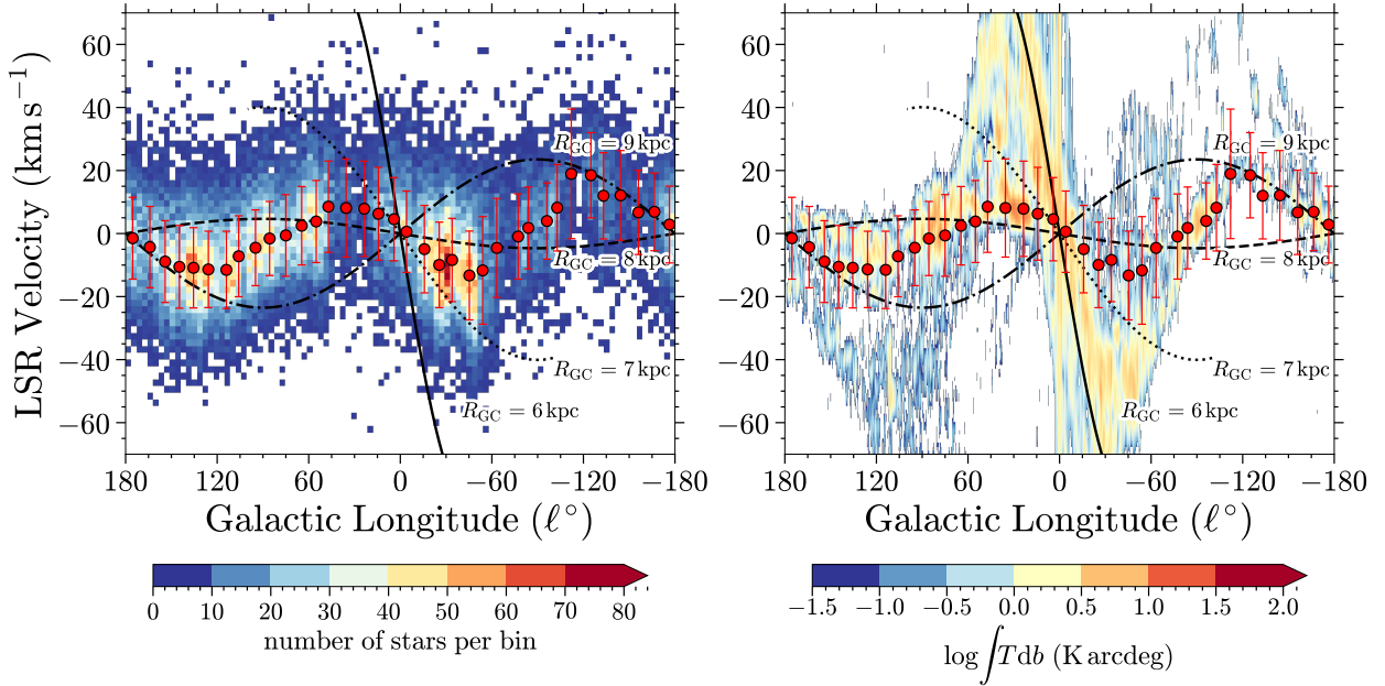
Fig. 17. (Left panel): Longitude–velocity diagram for the Gaia HQ DIB \lambda 862 sample. The circles indicate the median V_{\text{LSR}} and standard uncertainty of the mean for each field. Velocity curves calculated by Model A5 in Reid et al. (2019) for different galactocentric distances ( R_{\text{GC}} ) are overplotted. (Right panel): Same as left panel but superimposed on the ^{12}\text{CO} data from Dame et al. (2001). The colour-scale displays the ^{12}\text{CO} brightness temperature in a logarithmic scale integrated over the velocity range.
