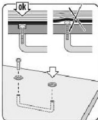
Countersink screw fittings of the hand grips.
