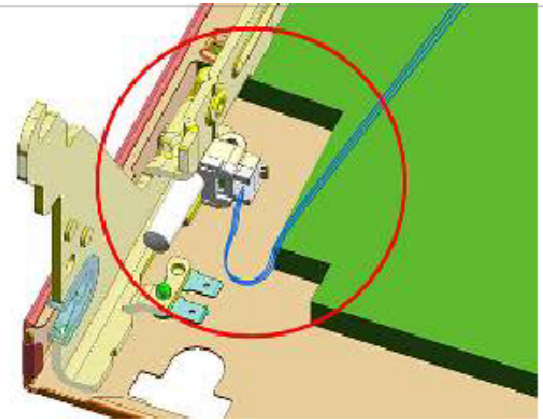
Illustration 2: Cut out damming mat from FD 8811on
