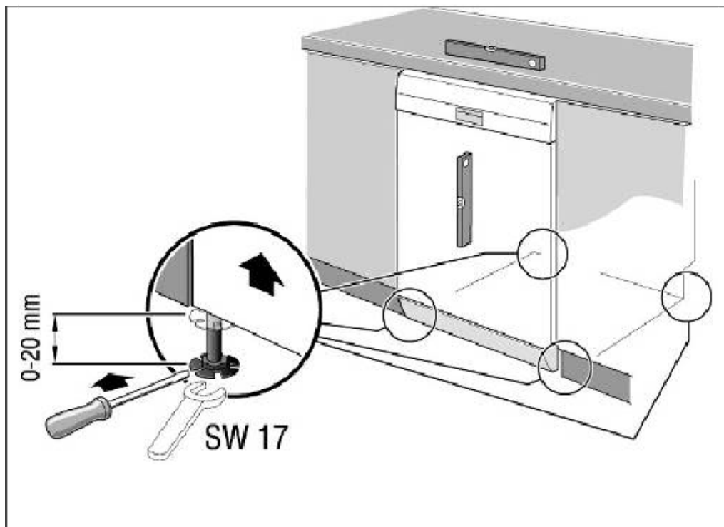
Illustration 1: Free-standing appliance
