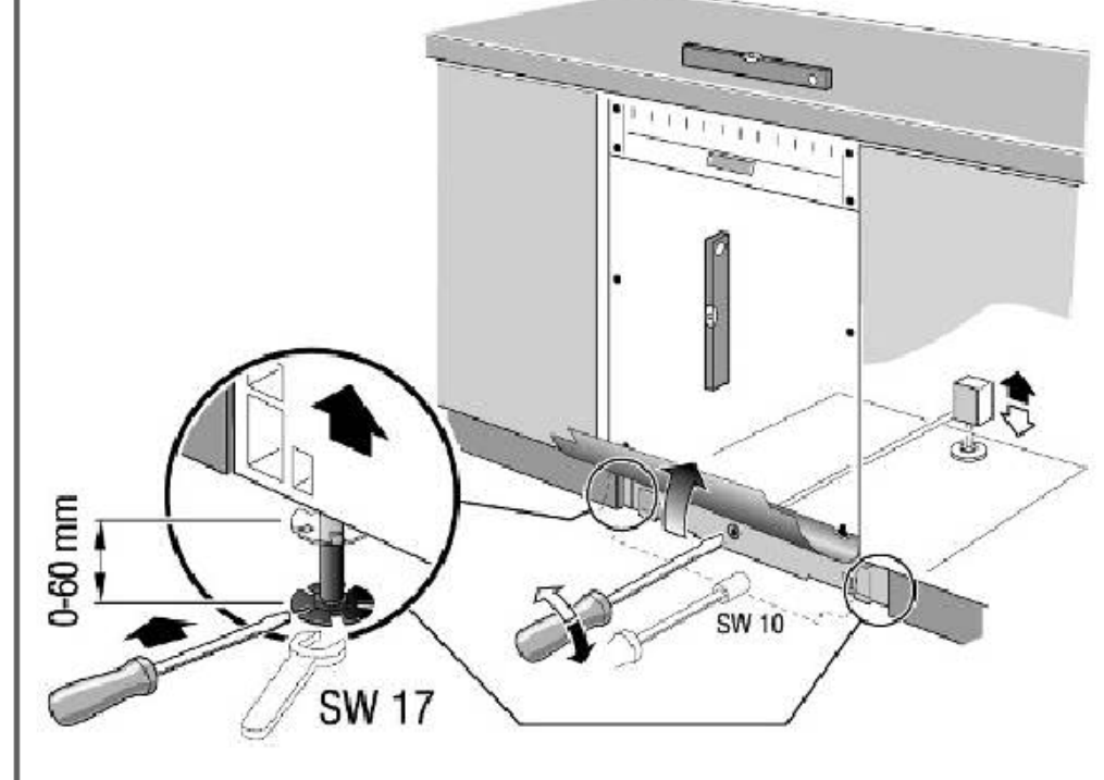
Illustration 2: Built-in & built-under appliance
