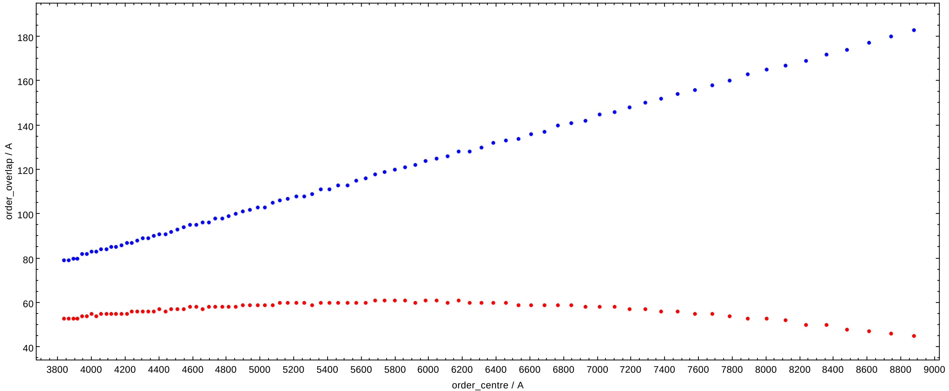
Wavelength dependency of order overlaps and order length
